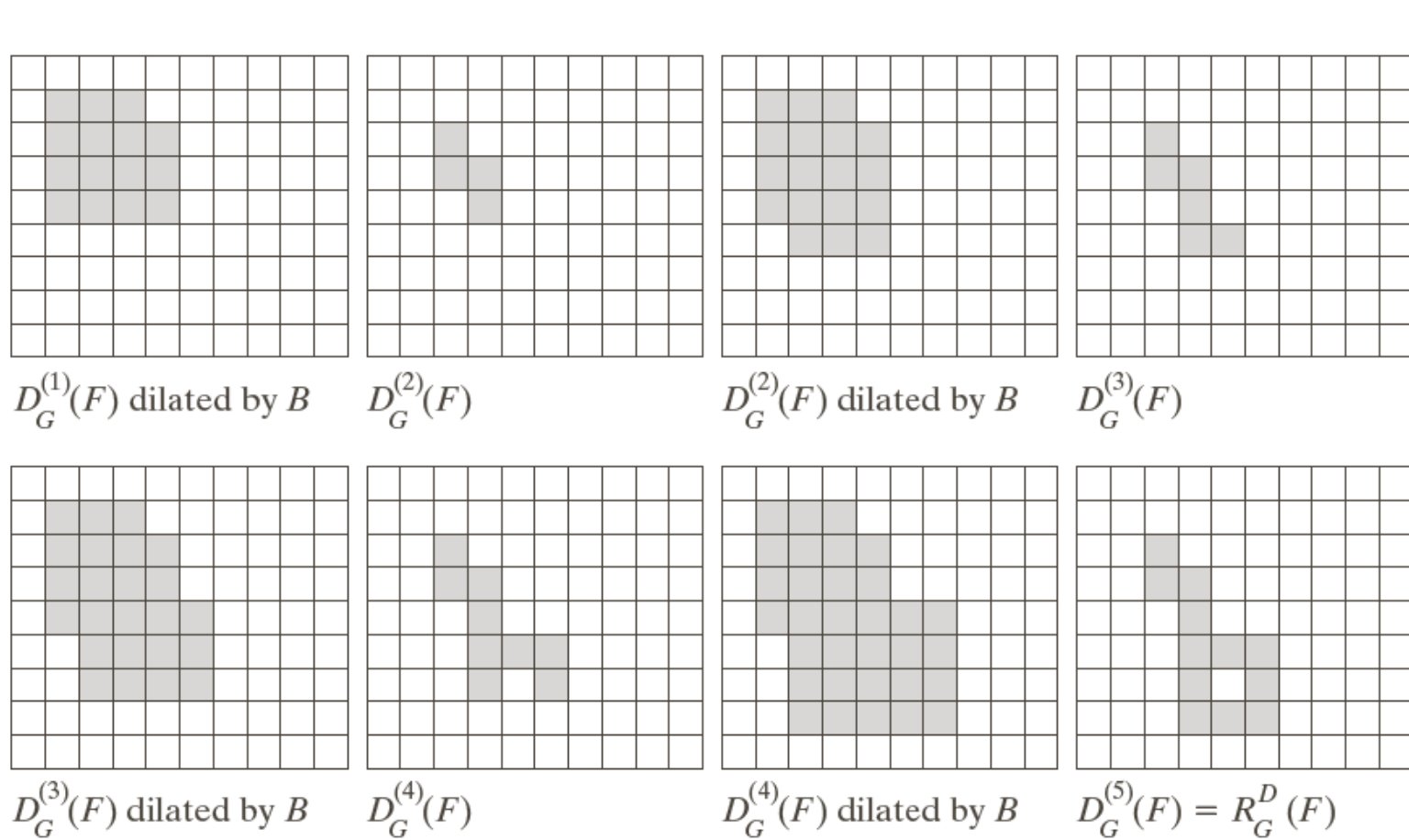
FIGURE 9.28 Illustration of morphological reconstruction by dilation. F , G , B and D_G^{(1)}(F) are from Fig. 9.26.
